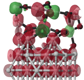
Magnetic oxide layer on cobalt
